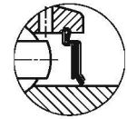
F seal (+Suffix-F)
