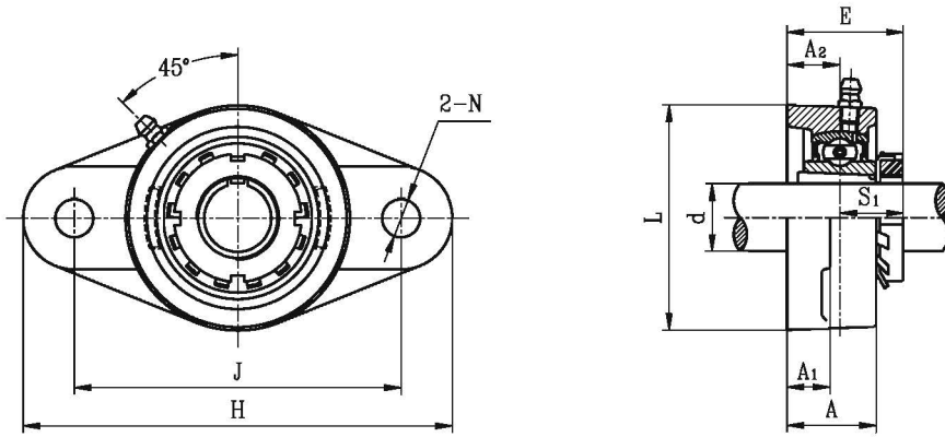
UKFL2+H Tapered bore, adapter type
