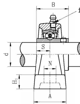
UCP200M Setscrew type
